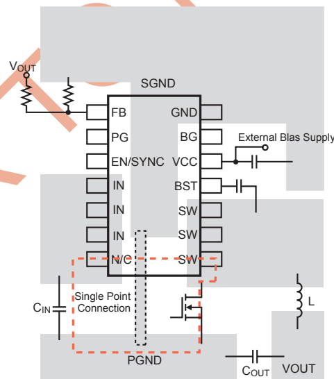
Figure 3—PCB Layout Conceptual Drawing, Only Top Layer Shown, and a Ground Plane Is Assumed
