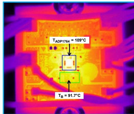
Figure 56. Thermal Image of the ADP1764 Evaluation Board at I LOAD = 4 A, V IN = 1.5 V, V OUT = 1.3 V, T B = 91.7°C
