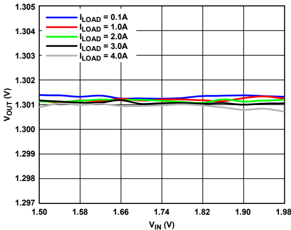
Figure 6. Output Voltage ( V_{OUT} ) vs. Input Voltage ( V_{IN} ), V_{OUT} = 1.3\text{ V}
