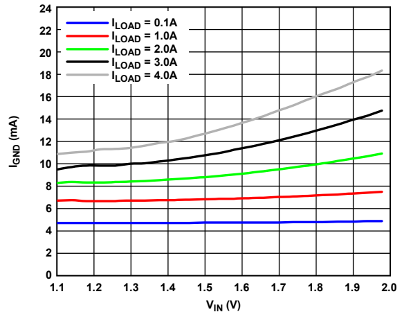
Figure 15. Ground Current ( I_{GND} ) vs. Input Voltage ( V_{IN} ), V_{OUT} = 0.9 V
