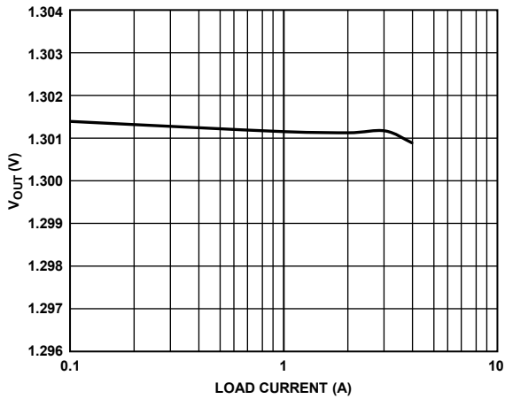
Figure 5. Output Voltage ( V_{OUT} ) vs. Load Current ( I_{LOAD} ), V_{OUT} = 1.3\text{ V}
