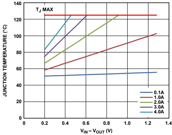
Figure 53. 6400 mm 2 of PCB Copper, T A = 50°C, LFCSP
