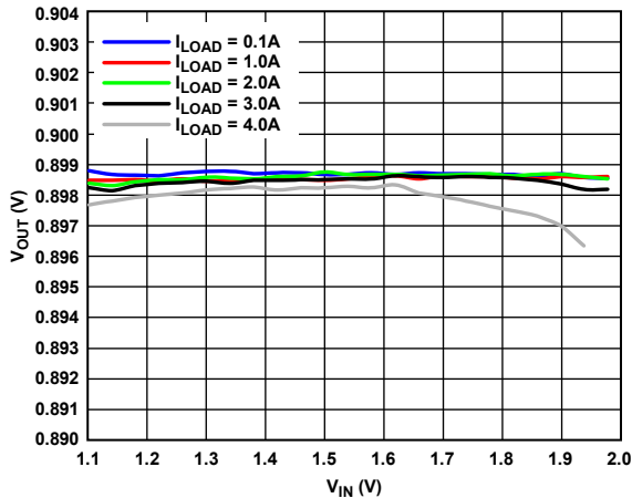
Figure 12. Output Voltage ( V_{OUT} ) vs. Input Voltage ( V_{IN} ), V_{OUT} = 0.9 V
