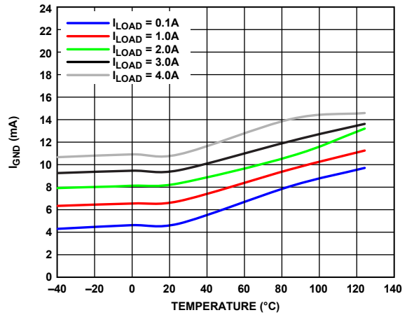
Figure 13. Ground Current ( I_{GND} ) vs. Temperature, V_{OUT} = 0.9 V
