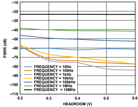
Figure 36. Power Supply Rejection Ratio (PSRR) vs. Headroom Voltage at Various Frequencies, V_{OUT} = 0.9 V , Load = 4 A
