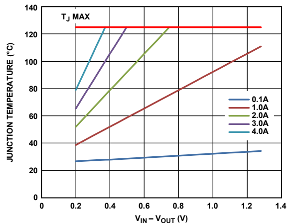
Figure 52. 500 mm 2 of PCB Copper, T_A = 25^\circ\text{C}
