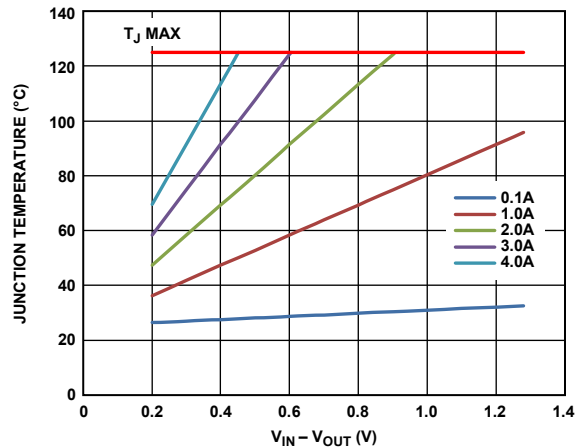
Figure 51. 1000 mm 2 of PCB Copper, T_A = 25^\circ\text{C}
