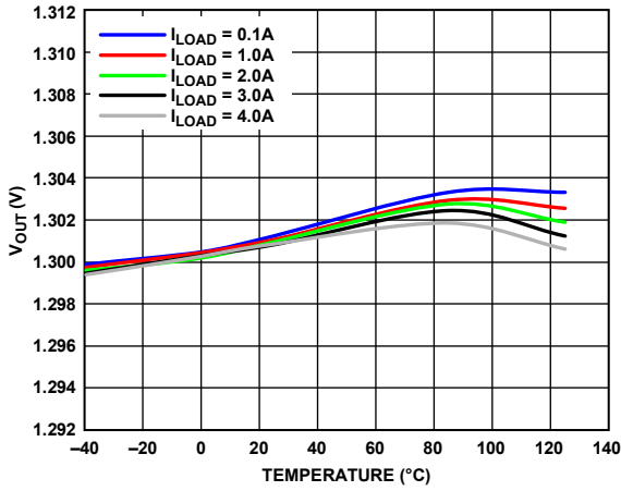
Figure 4. Output Voltage ( V_{OUT} ) vs. Temperature, V_{OUT} = 1.3\text{ V}
