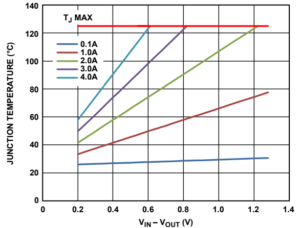
Figure 50. 6400 mm 2 of PCB Copper, T_A = 25^\circ\text{C}
