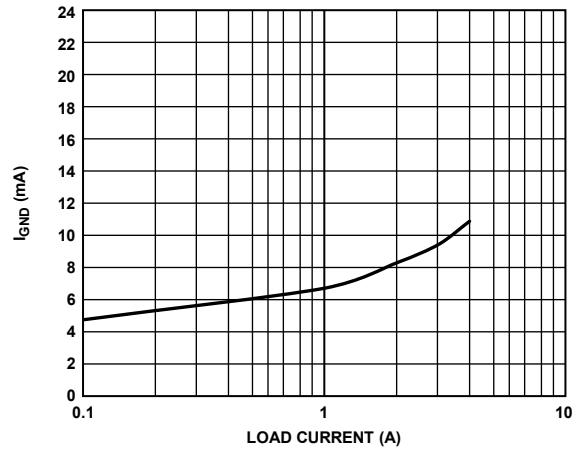
Figure 14. Ground Current ( I_{GND} ) vs. Load Current ( I_{LOAD} ), V_{OUT} = 0.9 V
