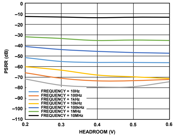
Figure 37. Power Supply Rejection Ratio (PSRR) vs. Headroom Voltage at Various Frequencies, V_{OUT} = 1.3 V , Load = 4 A
