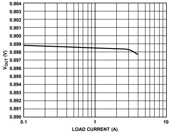
Figure 11. Output Voltage ( V_{OUT} ) vs. Load Current ( I_{LOAD} ), V_{OUT} = 0.9 V
