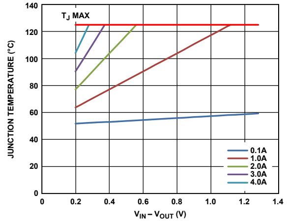
Figure 55. 500 mm 2 of PCB Copper, T A = 50°C, LFCSP
