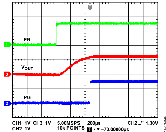
Figure 44. V_{OUT} vs. Typical PG Voltage Behavior, V_{IN} Rising ( V_{OUT} = 1.3 V)
