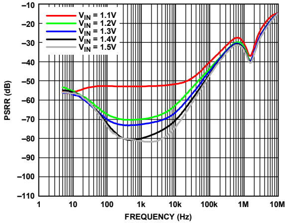
Figure 34. Power Supply Rejection Ratio (PSRR) vs. Frequency at Various Input Voltages ( V_{IN} ), V_{OUT} = 0.9 V , Load = 4 A
