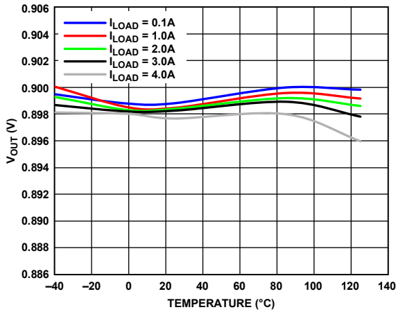
Figure 10. Output Voltage ( V_{OUT} ) vs. Temperature, V_{OUT} = 0.9 V
