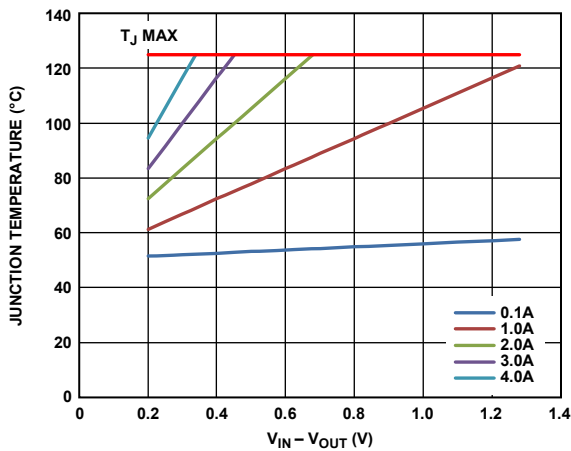
Figure 54. 1000 mm 2 of PCB Copper, T A = 50°C, LFCSP
