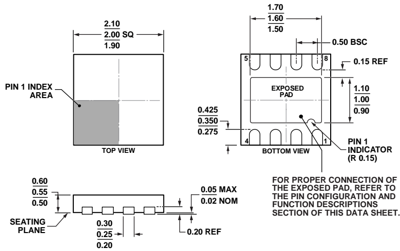
Figure 52. 8-Lead Lead Frame Chip Scale Package [LFCS_P_UD] 2.00 mm x 2.00 mm Body, Ultra Thin, Dual Lead (CP-8-10) Dimensions shown in millimeters
