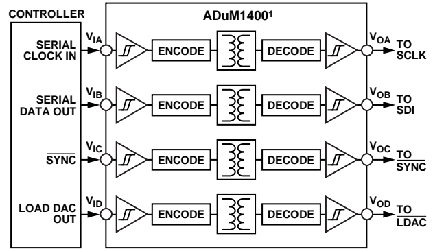
Figure 72. Isolated Interface
