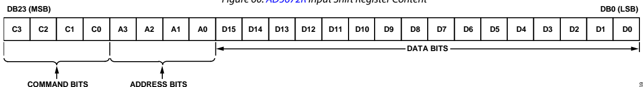
Figure 60. AD5672R Input Shift Register Content
