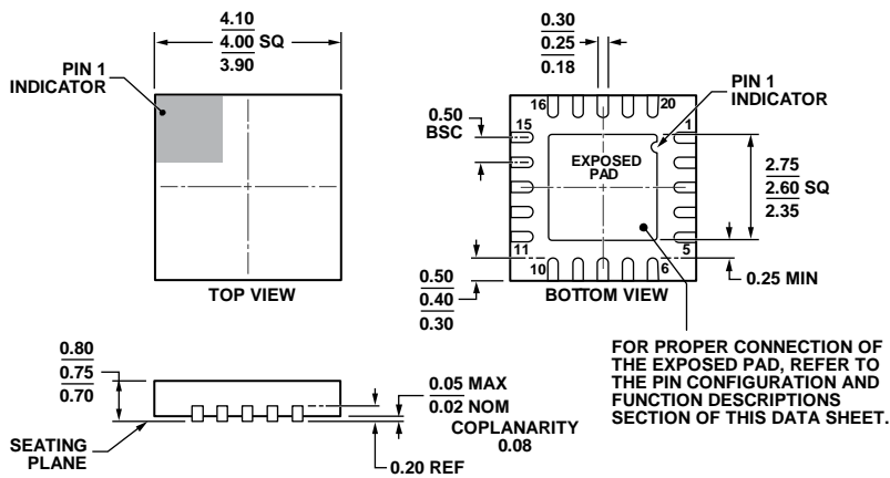
Figure 74. 20-Lead Lead Frame Chip Scale Package [LFCSP_WQ]
