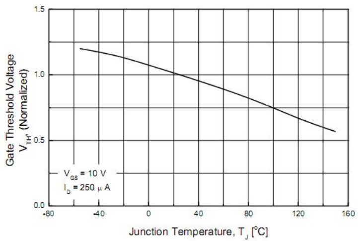
GP1M008A080FH
