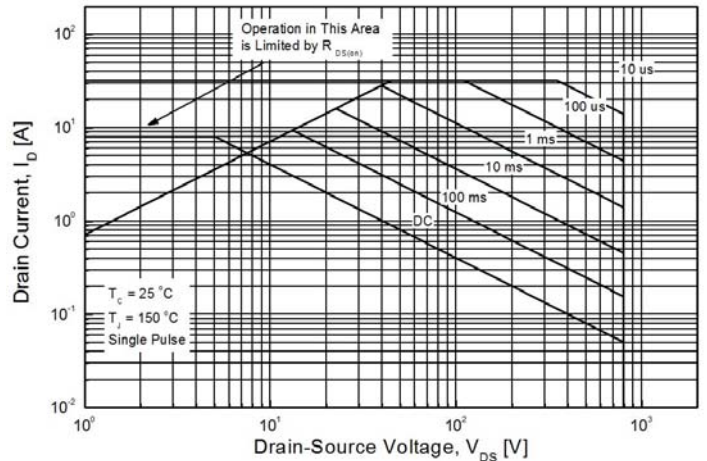
GP1M008A080FH
