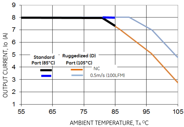
Figure 57. Derating Output Current versus Ambient Temperature and Airflow.
