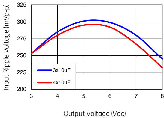
Figure 28. Input ripple voltage for various output voltages with 3 \times 10 \mu F or 4 \times 10 \mu F ceramic capacitors at the input (maximum load). Input voltage is 12V. Scope BW at 20MHz
