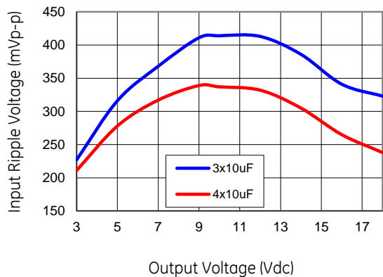
Figure 29. Input ripple voltage for various output voltages with 3 \times 10 \mu F or 4 \times 10 \mu F ceramic capacitors at the input (maximum load). Input voltage is 28V. Scope BW at 20MHz
