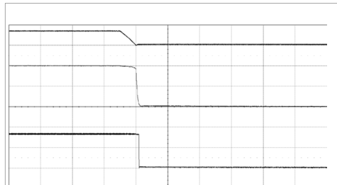
Disable by Input Voltage – PG Push-Pull
