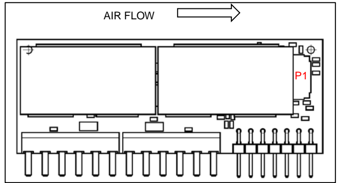
Temperature positions and air flow direction.
