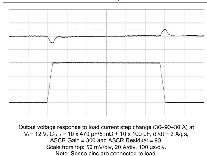
Transient Response
