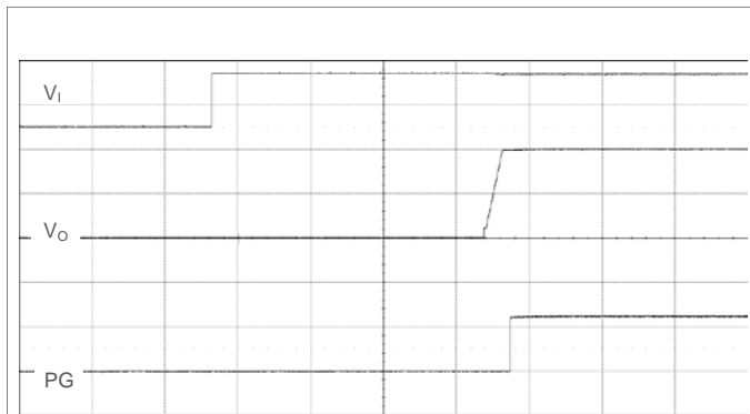
Enable by Input Voltage – PG Push-Pull
