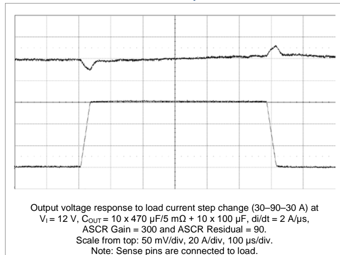
Transient Response
