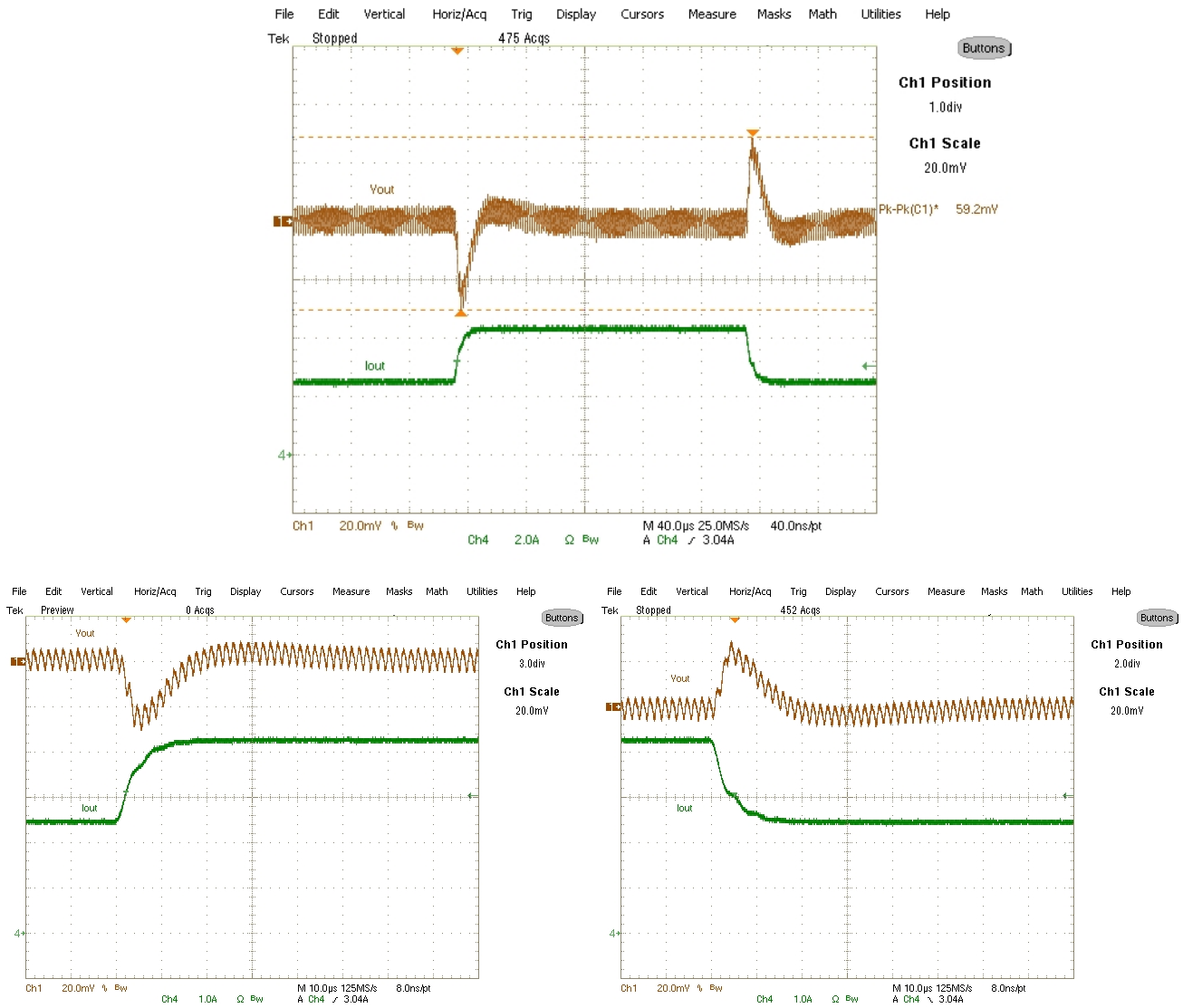
Fig. 15: Transient Response 2.4A-4.2A load (0.5A/ \mu s) Ch 1 : V_{out} , Ch 4 : i_o
