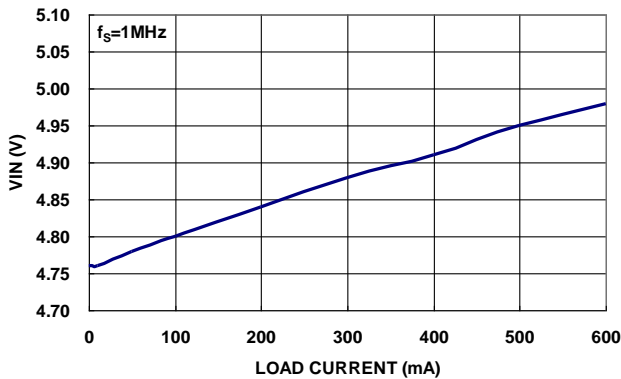
(b) V_{OUT}=5V
