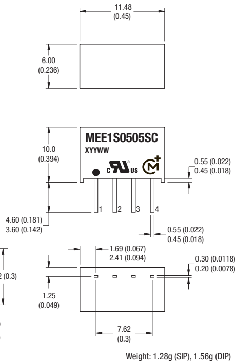
SIP Package
