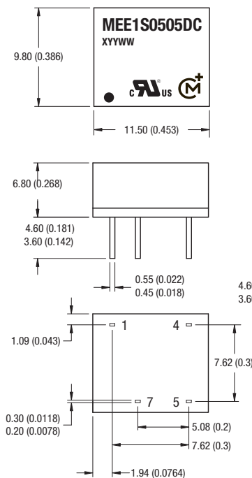
DIP Package
