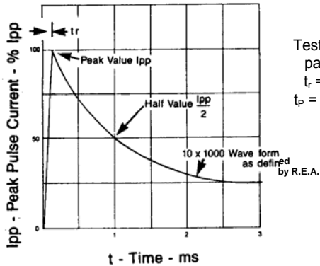
FIGURE 3 PULSE WAVEFORM
