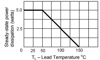
FIGURE 5 Steady-state power derating curve
