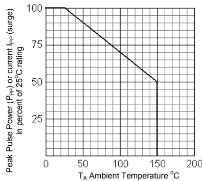
FIGURE 4 Derating curve
