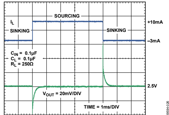
Figure 26. ADR3525 Load Transient Response
