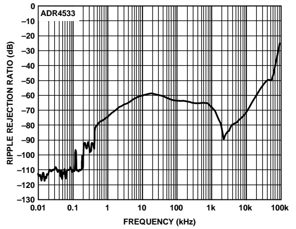
Figure 59. ADR4533 Ripple Rejection Ratio vs. Frequency
