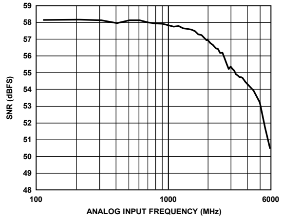
Figure 40. SNRFs vs. AIN Frequency at 2.5 GSPS (Input Network in Figure 76 Used <2 GHz, Input Network in Figure 75 Used >2 GHz)
