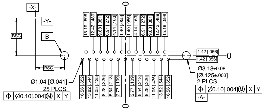
P.C. BOARD MOUNTING DIMENSIONS
