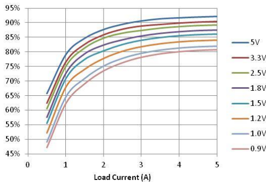
Figure 3. Efficiency vs. Load, V_{in}=12\text{V} , F_{sw}=500\text{KHz}
