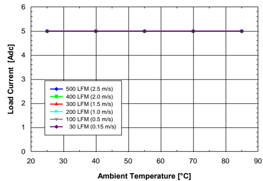
Figure 2. Available output current vs. ambient air temperature and airflow rates for converter DP8105G mounted horizontally with air flowing from input to output, MOSFET temperature \leq 120^\circ\text{C} , V_{in} = 12\text{V} , V_{out} = 5\text{V} , and F_{sw} = 1\text{MHz}
