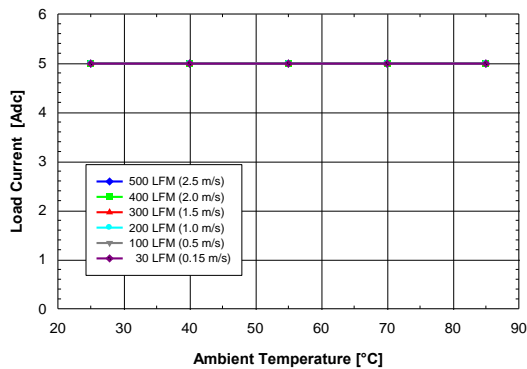
Figure 1. Available output current vs. ambient air temperature and airflow rates for converter DP8105G mounted horizontally with air flowing from input to output, MOSFET temperature \leq 120^\circ\text{C} , V_{in} = 12\text{V} , V_{out} = 5\text{V} , and F_{sw} = 500\text{KHz}
