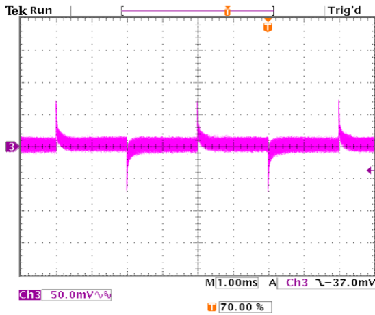
Figure 48. Transient Response with Regulation set to 0.0 mV/A.
