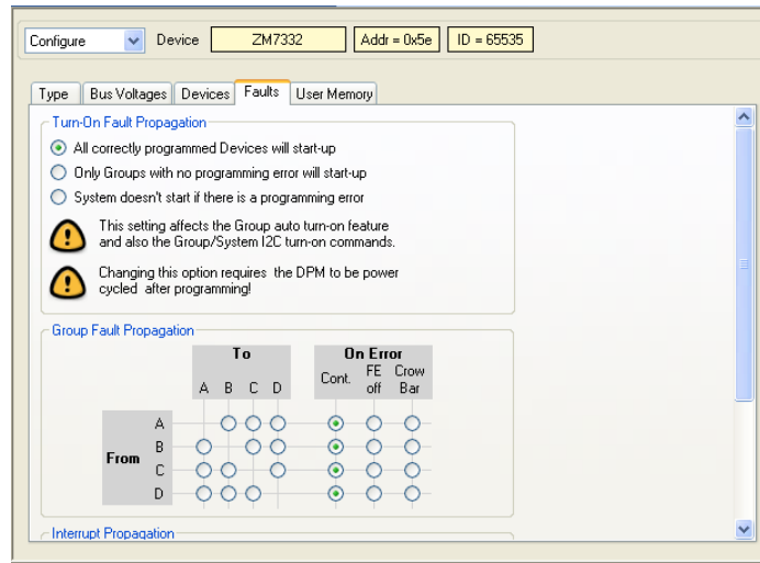
Figure 34. DPM Configure Faults Window
