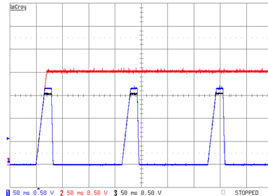
Figure 39. Turn-On into UVP on V3. The UV Fault Is Programmed To Be Non-Latching and Propagate From Group C to Group A. Ch1 – V3 (Group C), Ch2 – V2, Ch3 – V1 (Group A)
