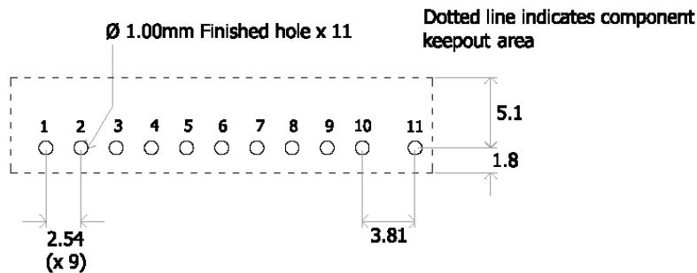
Figure 57. Recommended Footprint – Top View
