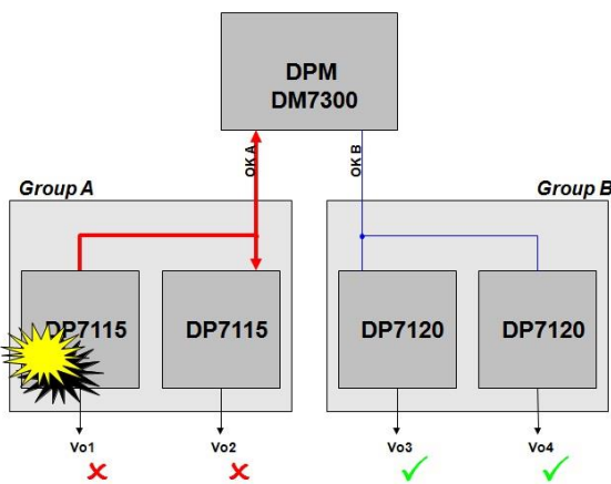
Figure 38. Intra Group Fault Propagation
