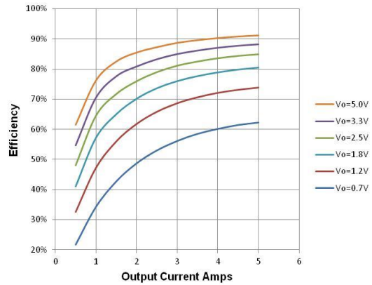
Figure 6. Efficiency vs Load, V_{in}=12V , F_{sw}=1MHz
