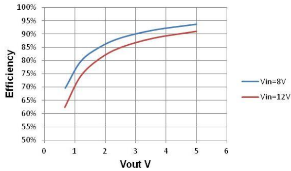
Figure 7. Efficiency vs Output Voltage, I_{out}=5A , F_{sw}=1MHz
