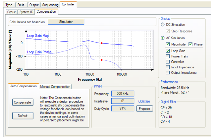
Figure 41. PWM Controller Window
