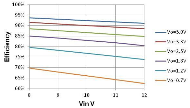
Figure 8. Efficiency vs Input Voltage at I_{out}=5A , F_{sw}=1MHz
