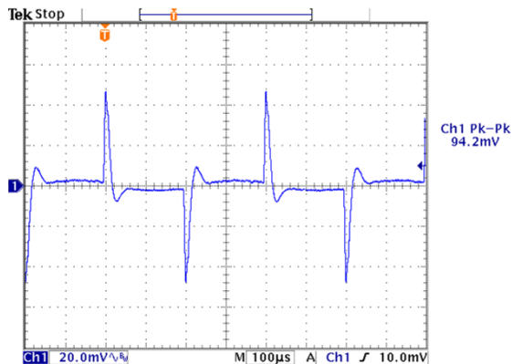
Figure 14 Transient Response with Regulation set to 0 mV/A.
