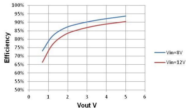
Figure 4. Efficiency vs. Output Voltage, I_{out}=5\text{A} , F_{sw}=500\text{kHz}
