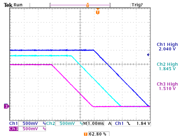
Figure 27. Turn-Off with Tracking and Sequencing. Falling Slew Rate is Programmed at 0.5V/ms.
