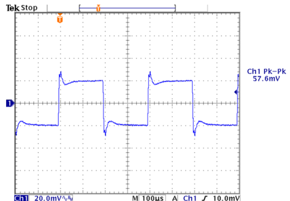
Figure 15 Transient response with non-zero Regulation.
