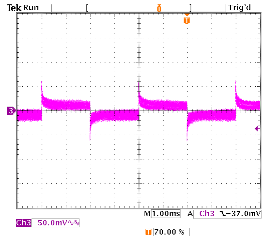
Figure 49. Transient Response with Regulation set to 6.53 mV/A.
