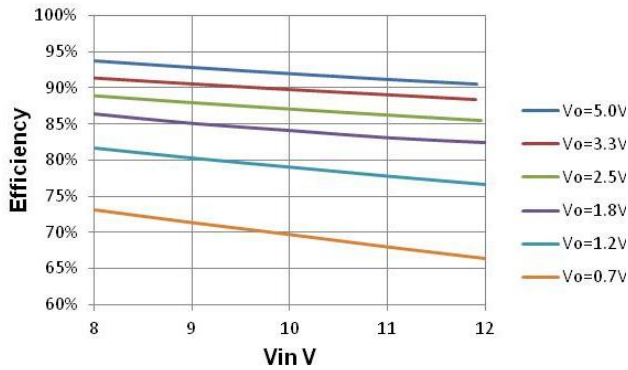
Figure 5. Efficiency vs Input Voltage at I_{out}=5A , F_{sw}=500KHz
