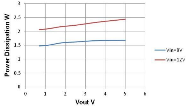
Figure 10. Power Dissipation vs Vout, I_{out}=5A , F_{sw}=1MHz
