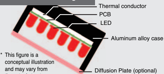
Cross-sectional Diagram
