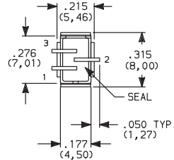
Terminal Nos. For Reference Only
