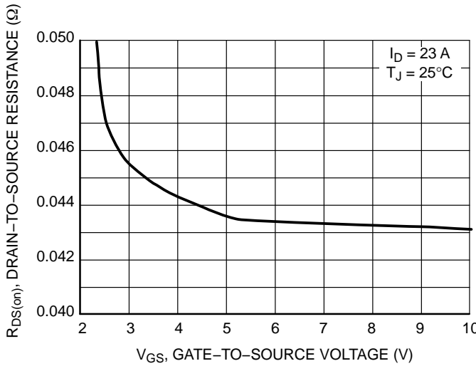
Figure 3. On-Resistance versus Gate Voltage
