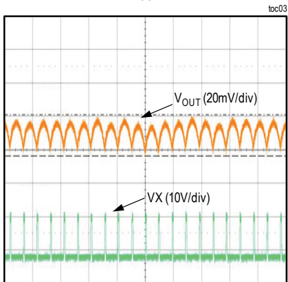
TIME: 5μs/div CONDITIONS: I_{OUT} = 40A
