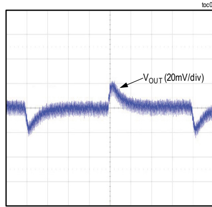
TIME: 50μs/div CONDITIONS: I_{OUT} = 20A to 30A STEP at 1A/\mu s
