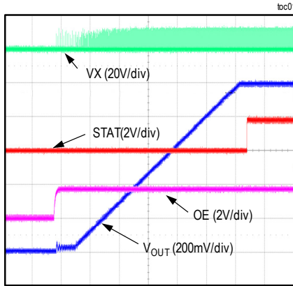
TIME: 500μs/div
