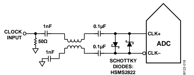
Figure 51. Balun-Coupled Differential Clock (Up to 625 MHz)
