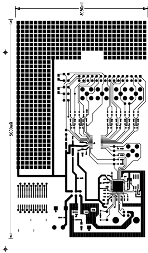
Figure 8. AD7795 Evaluation Board Component Side Artwork
