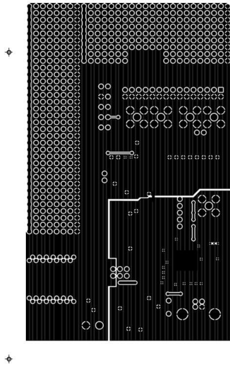
Figure 9. AD7795 Evaluation Board Solder Side Artwork
