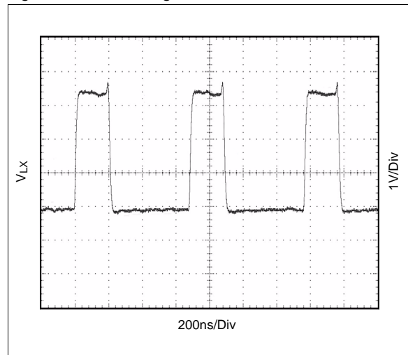
Figure 24. Coil Voltage, I_{OUT} = 100mA
