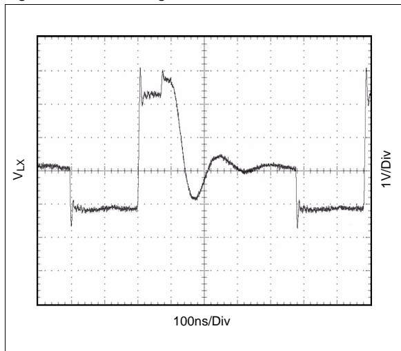
Figure 23. Coil Voltage, I_{OUT} = 1mA
