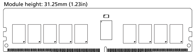
Figure 1: 288-Pin RDIMM (MO-309, R/C-C1)
