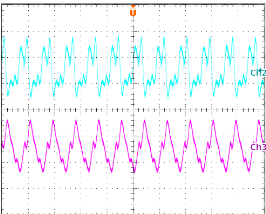
Output voltage ripple at nominal input voltage and max load current Top trace +15V, 10 mV/div, Bottom trace -15V, 20mV/div, 2μs/div. Load cap: 10μF, tantalum capacitor and 1μF ceramic capacitor. Bandwidth: 20 MHz.
