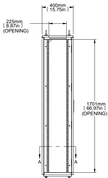
L.S. VIEW
