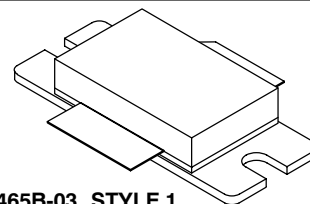
CASE 465B-03, STYLE 1 NI-880 MRF6S18140HR3
