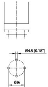
Direct Mounting
