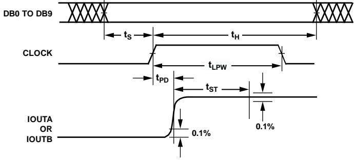
Figure 2. Timing Diagram
