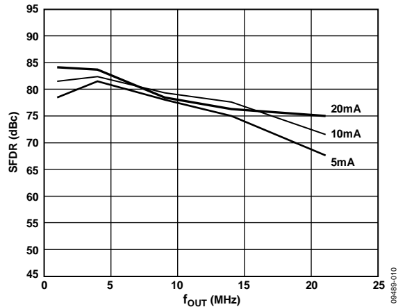
Figure 9. SFDR vs. f_{OUT} and I_{OUTFS} at 65 MSPS and 0 dBFS
