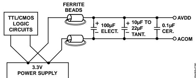
Figure 35. Differential LC Filter for Single 3.3 V Applications
