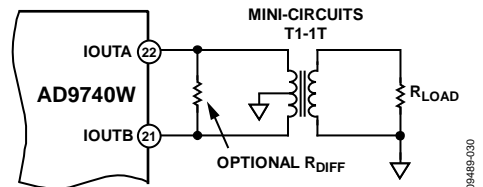
Figure 29. Differential Output Using a Transformer
