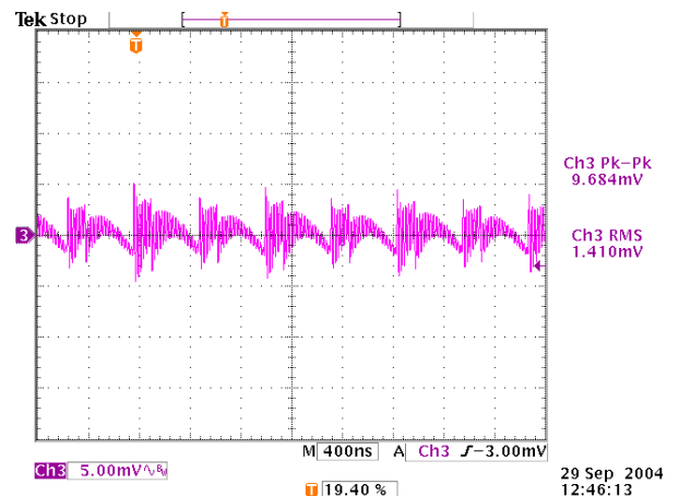
Figure 50. Output Voltage Noise, Full Load, 180° Interleave
