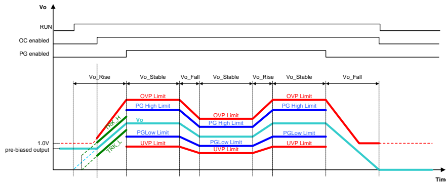
Figure 34. Protection Enable Conditions
