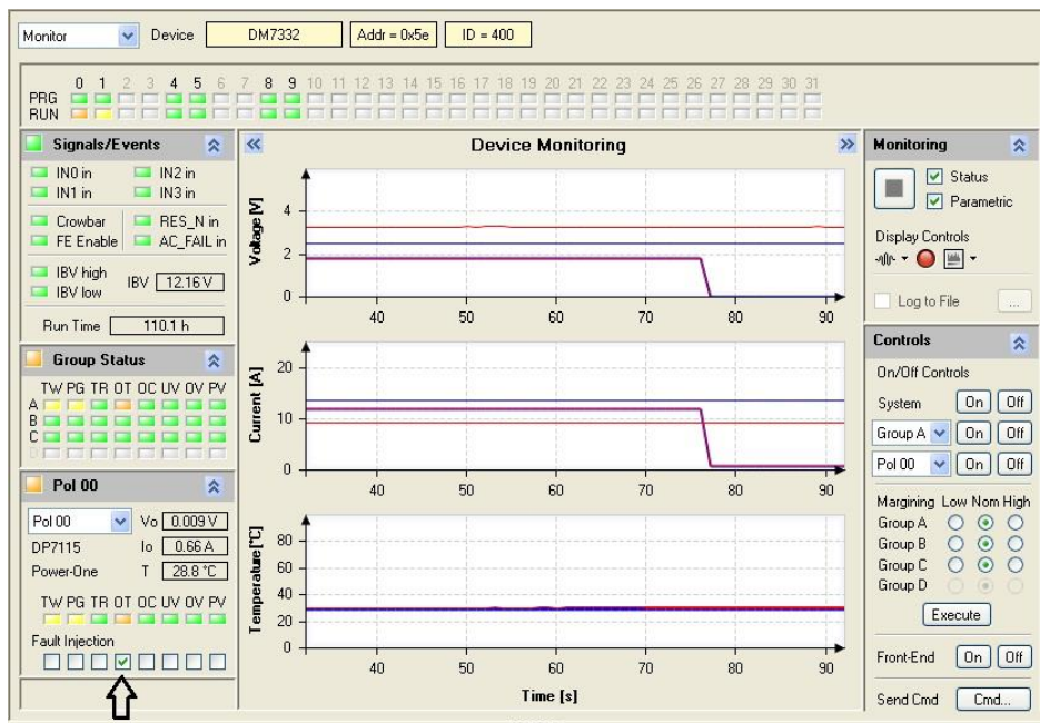
Figure 57. Example Overtemp Fault Injection in the GUI
