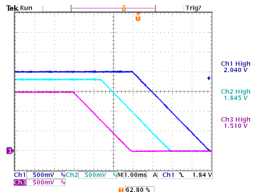
Figure 31. Turn-Off with Tracking and Sequencing. Falling Slew Rate is Programmed at 0.5V/ms.
