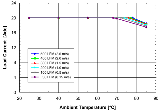
Figure 3. Available output current vs. ambient air temperature and airflow rates for converter DP7120G mounted horizontally with air flowing from input to output, MOSFET temperature \leq 120^{\circ}\text{C} , V_{in} = 12\text{ V} , V_{out} = 5\text{ V} , and F_{sw} = 500\text{KHz}
