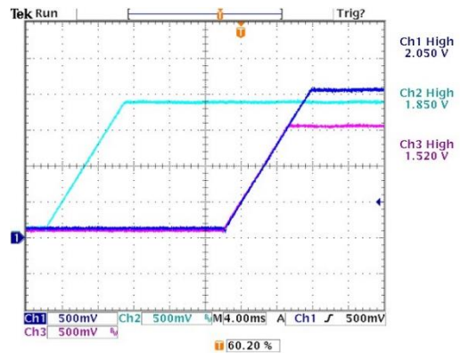
Figure 28 Two outputs delayed 5ms. All slew rates at 0.5V/ms
