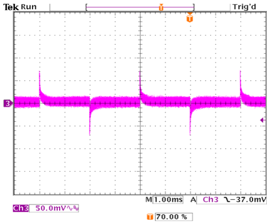
Figure 52. Transient Response with Regulation set to 0.0 mV/A.
