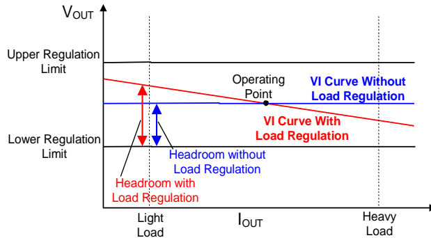
Figure 17. Optimal Voltage Positioning Concept
