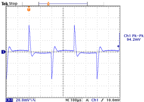
Figure 18 Transient Response with Regulation set to 0 mV/A.
