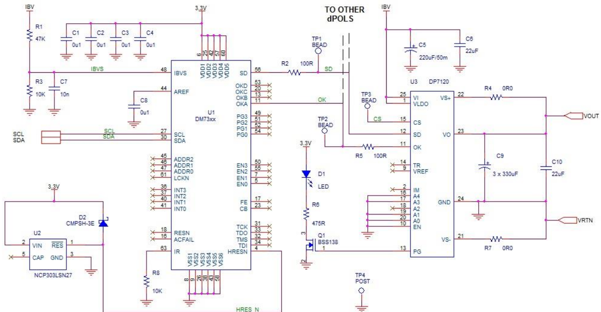
Figure 59. Typical Application with Digital Power Manager and I2C Interface
