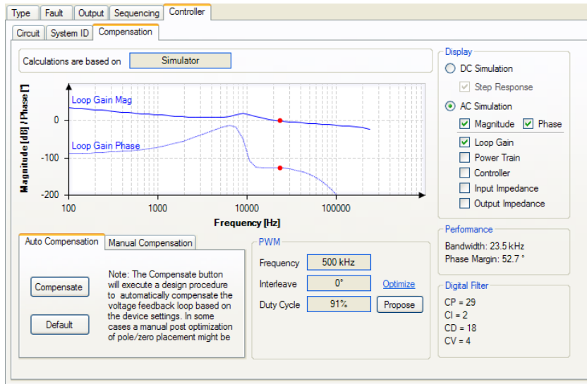
Figure 45. PWM Controller Window
