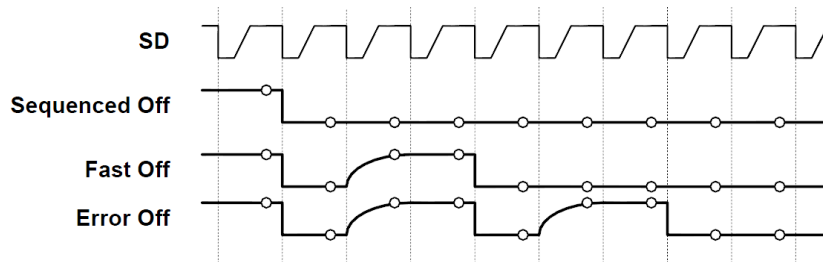
Figure 44. OK Severity Encoding Waveforms
