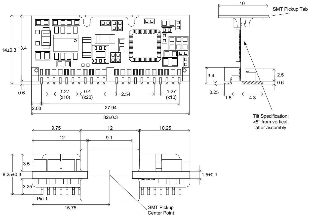
Figure 60. Mechanical Drawing
