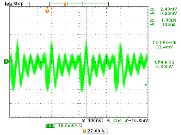
Figure 48. Input Voltage Noise with Interleave
