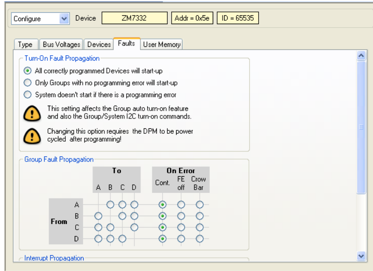
Figure 38. DPM Configure Faults Window
