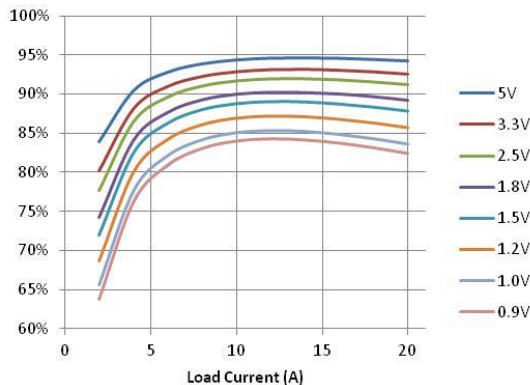
Figure 5. Efficiency vs. Load. V_{in} = 12\text{V} , F_{sw} = 500\text{KHz}
