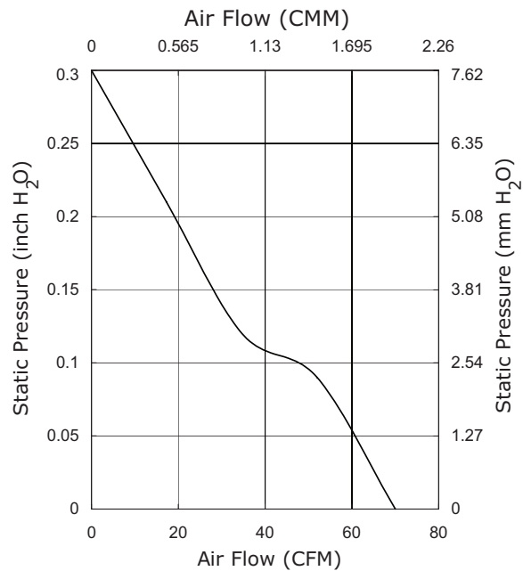
CFM-9225V-224-280
