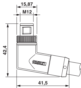
Dimensional drawing
