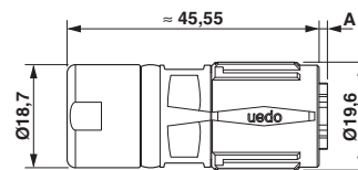
Dimensional drawing
