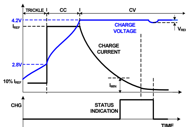
FIGURE 1. TYPICAL CHARGE CYCLE WITH TIMEOUT
