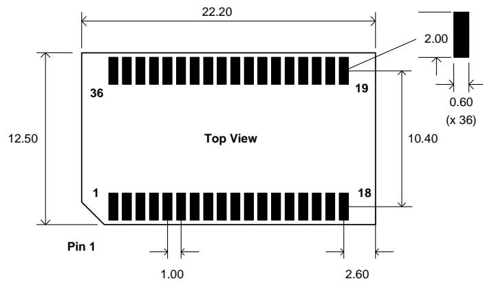
Figure 54. Recommended PCB Pad Sizes
