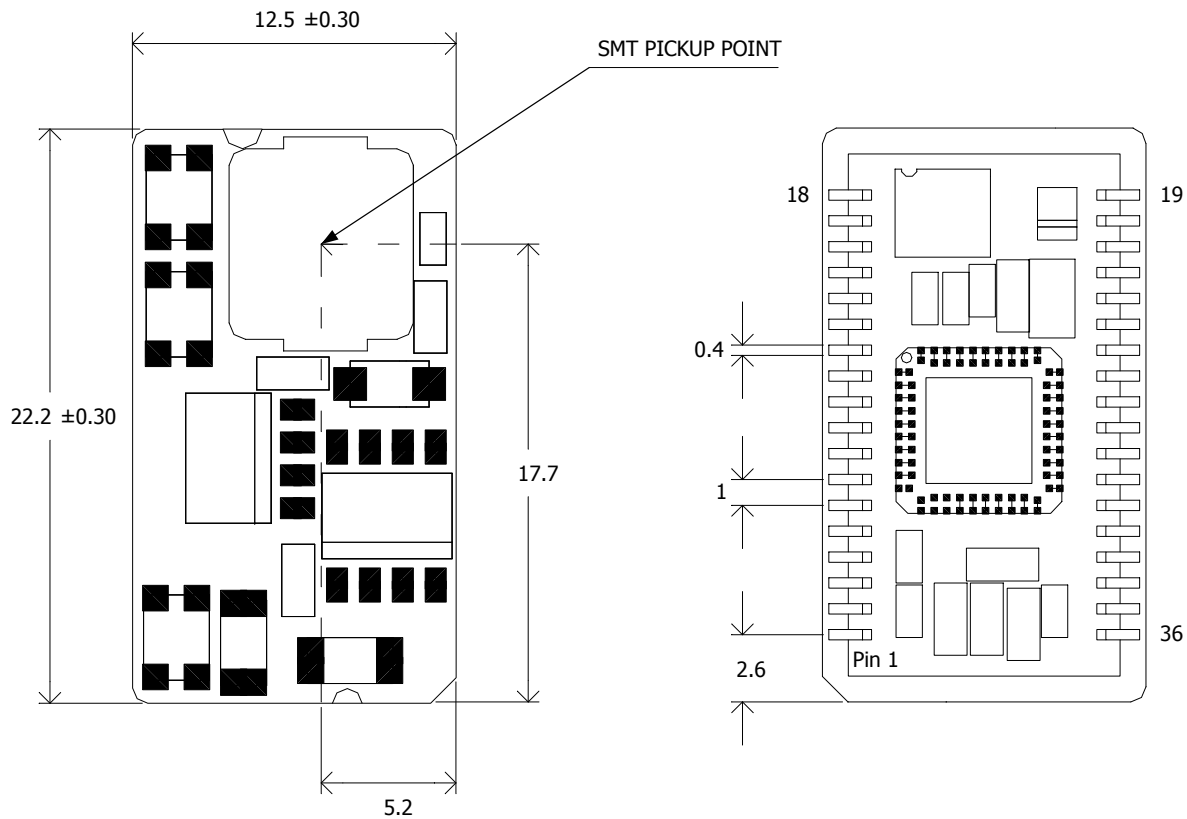
Figure 51. Top (Left) and Bottom Views
