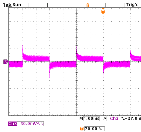
Figure 44. Transient Response with Regulation set to 3.72 mV/A.
