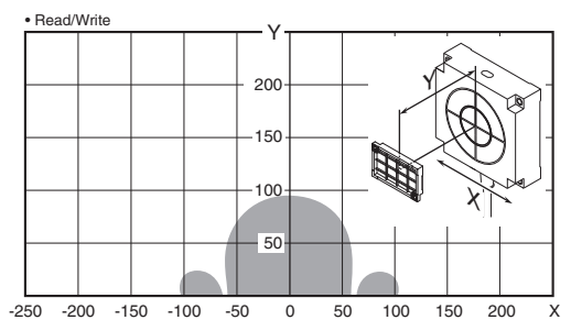
V680-HS65 (mounted on metallic surface: steel) & V680S-D8KF68M (Tag direction: Horizontal)
