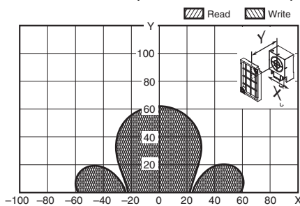
V680-HS65 (with Metal on Back Surface) & V680S-D2KF68M (Metal on back: Steel) (Tag direction: Vertical)
