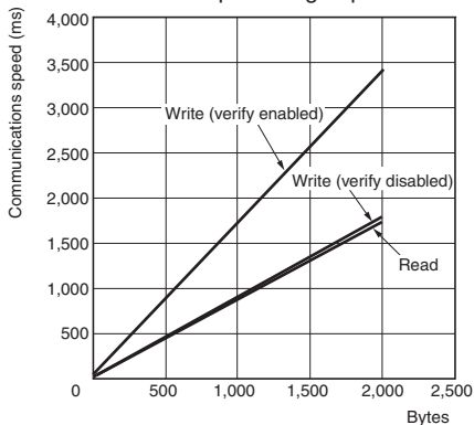
● Communications speed: High-speed mode
