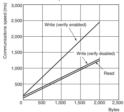
● Communications speed: Normal mode
