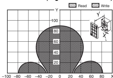
V680-HS65 (with Metal on Back Surface) & V680S-D2KF68 (Tag direction: Vertical)
