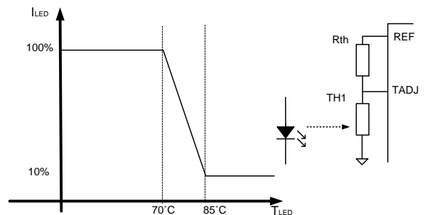
Thermal network response in Buck configuration with: R_{th} = 1.8k\Omega and TH1 = 10k\Omega ( \beta = 3900 )
