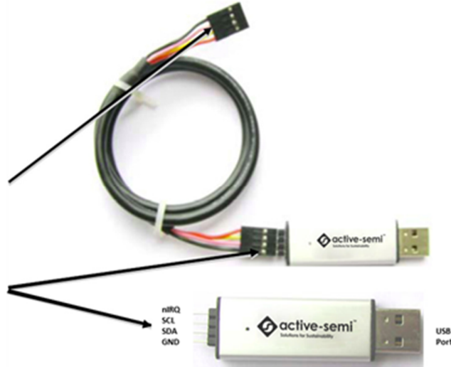
Figure 4 – USB-TO-I2C Dongle Connection
