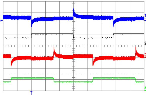
Figure 27. Output voltage response to both I_{out1} and I_{out2} (out of phase) load current step-change of 3.75 A (50%-75%-50%) at V_{in} = 48 V. Ch1 = V_{out1} (50 mV/div), Ch2 = V_{out2} (50 mV/div), Ch3 = I_{out1} (10 A/div.), Ch4 = I_{out2} (10 A/div.). Current slew rate: 0.1 A/ \mu s, C_o = 300 \mu F tantalum + 1 \mu F ceramic. Time scale: 1.0 ms/div.
