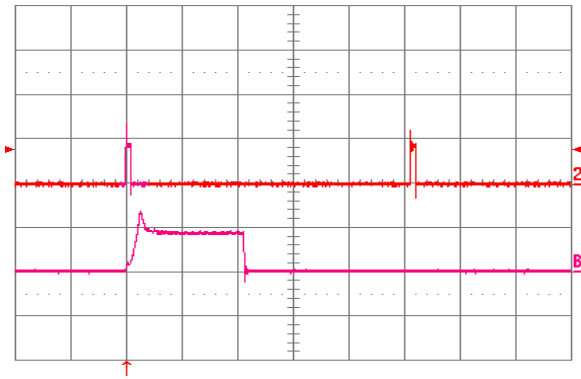
Figure 33. Load current i_{out1} into a 10\text{ m}\Omega short circuit on V_{out1} during re-start, with V_{out2} open (no load), at V_{in} = 48\text{ V} . Ch2 = i_{out1} ( 20\text{ A/div} , 20\text{ ms/div} ). ChB = i_{out1} ( 20\text{ A/div} , 1\text{ ms/div} ) is an expansion of the on-time portion of i_{out1} .
