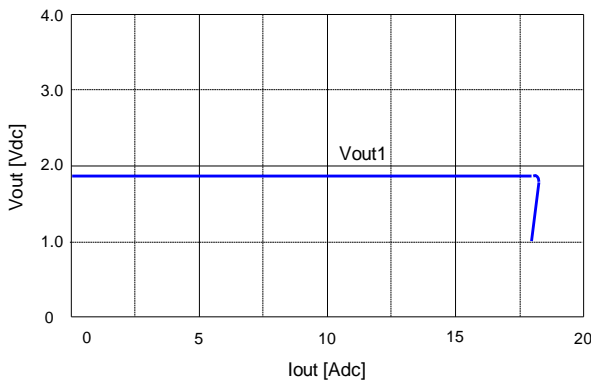
Figure 29. Output voltage V_{out1} vs. load current I_{out1} showing current limit point and converter shutdown point. When V_{out1} is in current limit, V_{out2} is not affected until V_{out1} reaches the shutdown threshold of 1 V. Input voltage has almost no effect on V_{out1} current limit characteristic.
