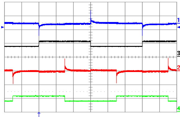
Figure 28. Output voltage response to both I_{out1} and I_{out2} (out of phase) load current step-change of 3.75 A (50%-75%-50%) at V_{in} = 48 V. Ch1 = V_{out1} (100 mV/div), Ch2 = V_{out2} (100 mV/div), Ch3 = I_{out1} (10 A/div.), Ch4 = I_{out2} (10 A/div.). Current slew rate: 5 A/ \mu s, C_o = 300 \mu F tantalum + 1 \mu F ceramic. Time scale: 1.0 ms/div.
