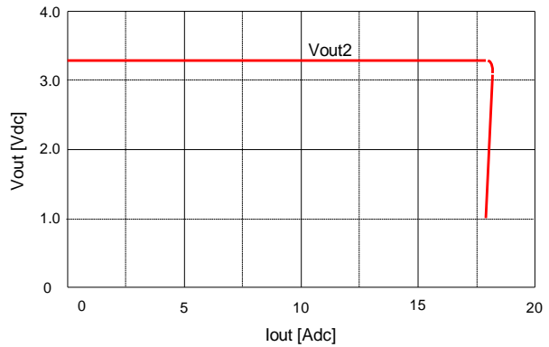
Figure 30. Output voltage V_{out2} vs. load current I_{out2} showing current limit point and converter shutdown point. When V_{out2} is in current limit, V_{out1} will follow with less than 0.6 V difference until shutdown threshold of 1 V. Input voltage has almost no effect on V_{out2} current limit characteristic.
