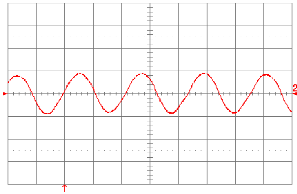
Figure 35. Input reflected ripple current, i_c ( 100\text{ mA/div} ), measured at input terminals at full rated load current on both outputs and V_{in} = 48\text{ V} . Refer to Fig. 34 for test setup. Time scale: 1\text{ }\mu\text{s/div} .
