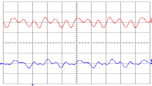
Figure 31. Output voltage ripple at full rated load current into a resistive load on both outputs with C_o = 1 \mu F (ceramic) and V_{in} = 48 V. Ch2 = V_{out2} , Ch1 = V_{out1} (both 20 mV/div). Time scale: 1 \mu s/div.
