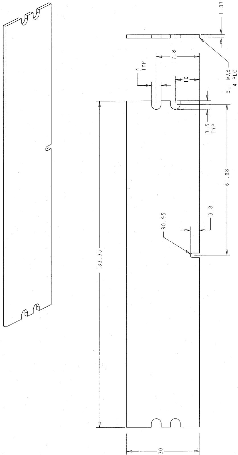
Figure 6 Steel Gage
