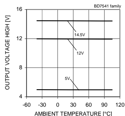
Fig. 52 Output Voltage High - Ambient Temperature ( R_L=10[k\Omega] )
