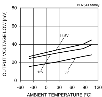
Fig. 54 Output Voltage Low - Ambient Temperature ( R_L=10[k\Omega] )
