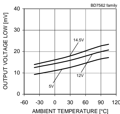
Fig. 31 Output Voltage Low - Ambient Temperature (RL=10[kΩ])
