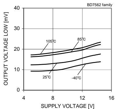
Fig. 30 Output Voltage Low - Supply Voltage (RL=10[kΩ])
