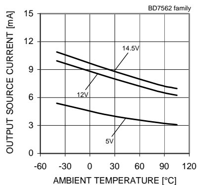
Fig. 33 Output Source Current - Ambient Temperature
