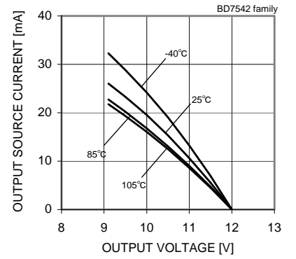
Fig. 78 Output Source Current - Output Voltage (VDD=12[V])
