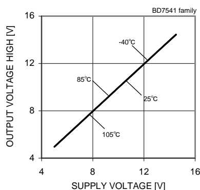
Fig. 51 Output Voltage High - Supply Voltage ( R_L=10[k\Omega] )
