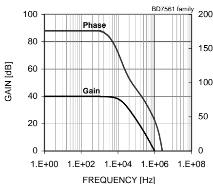
Fig. 23 Gain - Frequency
