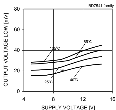
Fig. 53 Output Voltage Low - Supply Voltage ( R_L=10[k\Omega] )
