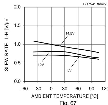
Slew Rate L-H – Ambient Temperature
