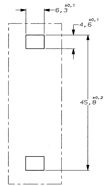
PANEL (1,4 MAX. TH.) CUT-OUT
