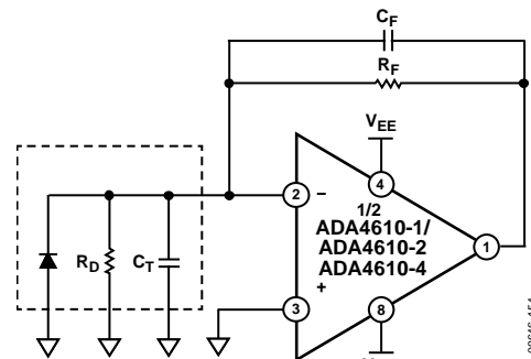
Figure 59. Equivalent Preamplifier Photodiode Circuit
