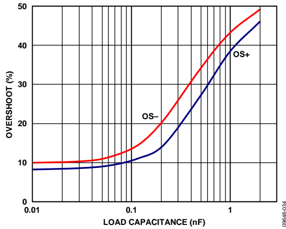
Figure 40. Overshoot vs. Load Capacitance, V_{SV} = \pm 5 V , A_V = +1 , R_L = 2 k\Omega , V_{IN} = 100 mV p-p
