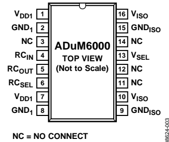
Figure 3. Pin Configuration
