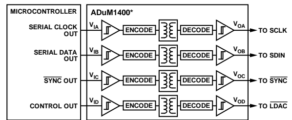
Figure 66. Isolated Interface
