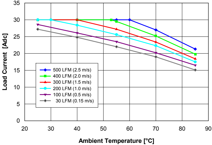
Fig. 12: Available load current vs. ambient temperature and airflow rates for converter mounted horizontally with V_{in} = 54\text{ V} , air flowing from pin 3 to pin 4 and maximum FET temperature \leq 120^{\circ}\text{C} .
