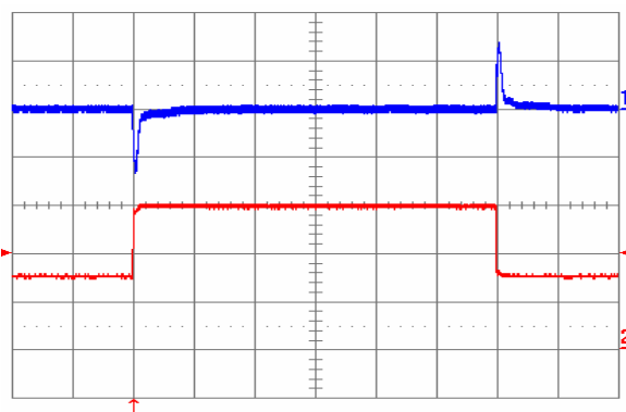
Fig. 21: Output voltage response to load current step-change (7.5 A – 15 A – 7.5 A) at V_{in} = 48\text{ V} . Top trace: output voltage (100 mV/div). Bottom trace: load current (5 A/div.). Current slew rate: 5 A/ \mu\text{s} . C_o = 450\ \mu\text{F} tantalum + 1 \mu\text{F} ceramic. Time scale: 0.2 ms/div.
