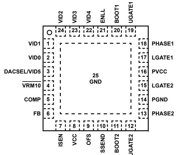
ISL6315 (24 LD QFN) TOP VIEW
