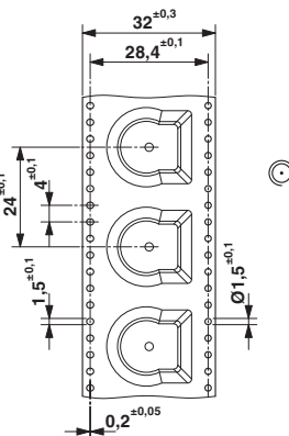
THR tape-on-reel packing
