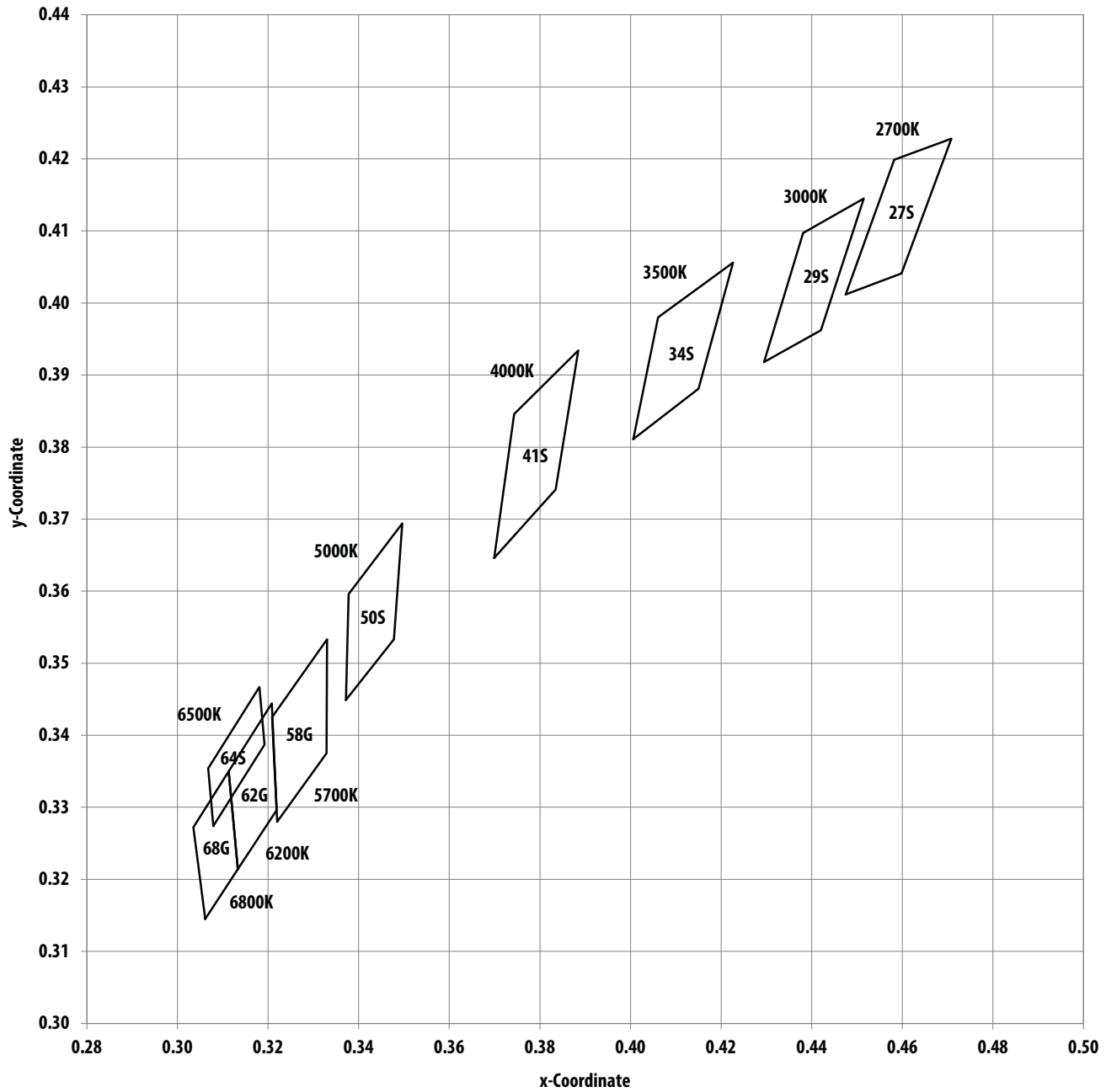
Figure 2 Chromaticity Diagram
