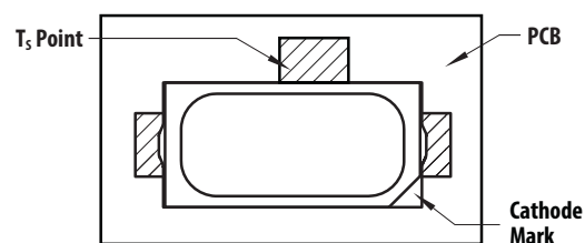
Figure 21 Solder Point Temperature on the PCB
