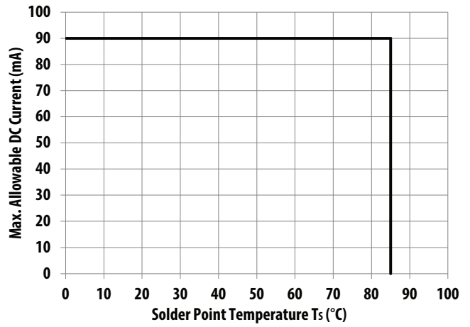
Figure 16 Maximum Forward Current vs. Solder Point Temperature. Derated based on T_{JMAX} = 110^{\circ}C , R\theta_{J-S} = 46^{\circ}C/W .
