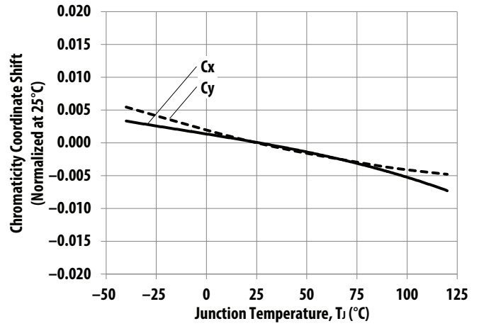
Figure 13 Chromaticity Coordinate Shift vs. Junction Temperature for 4000K
