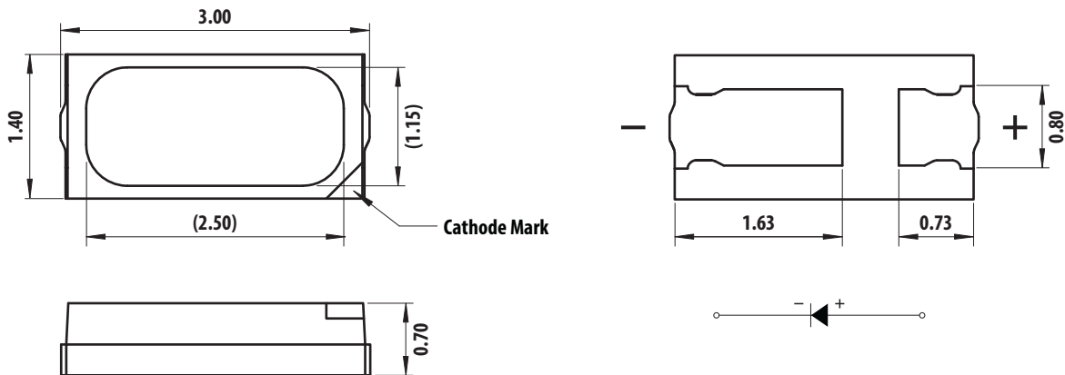
Figure 1 Package Drawing
