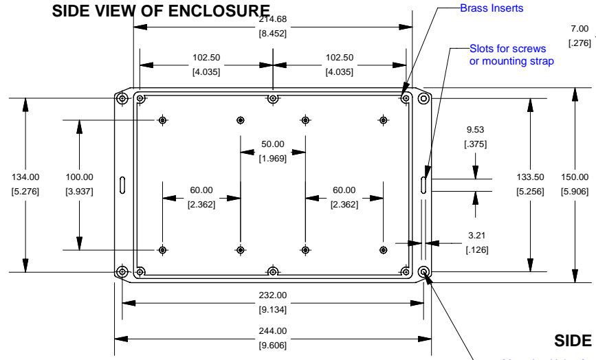
BOTTOM VIEW OF LID
